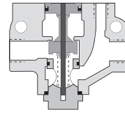
3/2 Normal offen
