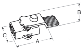
PEDAL
